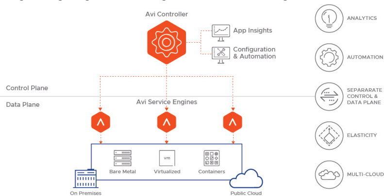
FIGURE 1: NSX Advanced Load Balancer High-level Architecture
